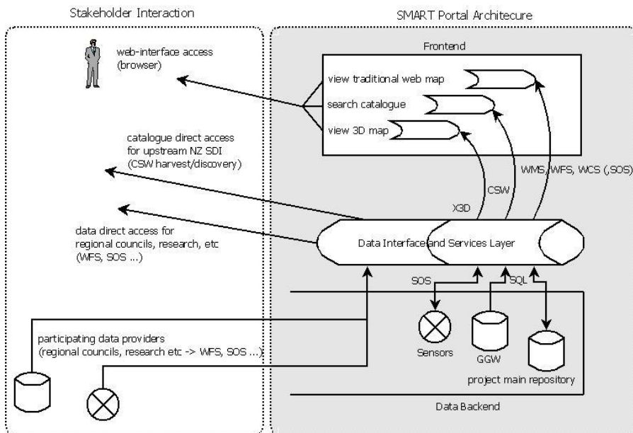
Fig. 2: SMART Portal architecture overview and stakeholder interaction
