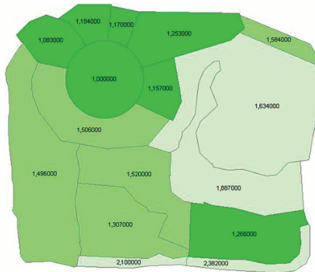
Fig. 2. Shape index for patches of various forms. The ranking shows values from 1 to 1.5 (dark shades), 1.5 to 2 (medium shades), beyond 2 (bright shades).
