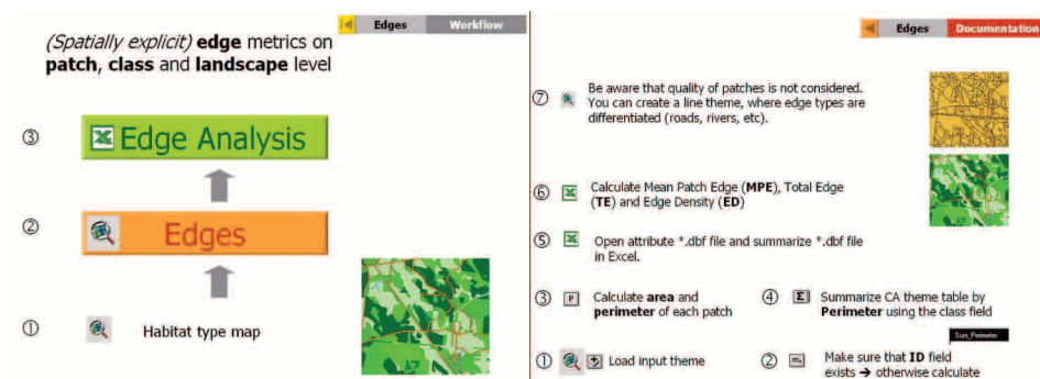
Fig. 1. User interface of the IMT with control buttons (example: 'edges'). Overview of workflow (left) and detailed descriptions of steps to be performed (right).
